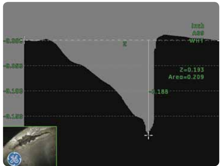
Profile View
